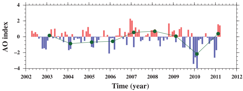
Figure 1. Time-series of the monthly AO index from National Oceanic and Atmospheric Administration ( http://www.cpc.ncep.noaa.gov/products/precip/CWlink/daily_ao_index/ao.shtml ). Red and blue bars show positive and negative phases of AO, respectively. The green curve shows the time series of the three month (JFM) averages of AO indices in NH winters.
