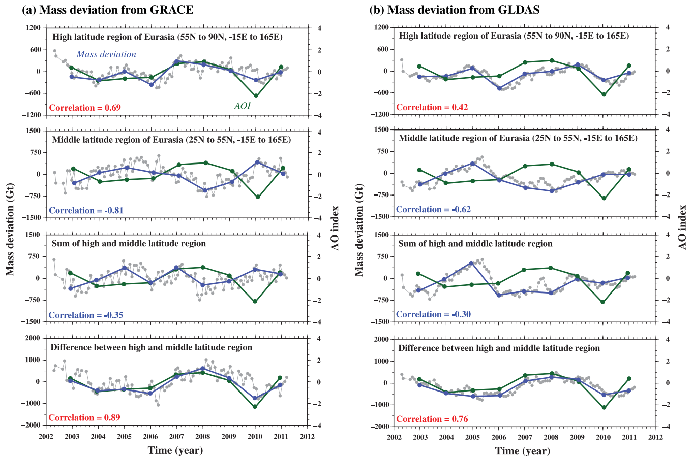
Figure 6. From top to bottom, time-series of mass deviation in high latitude region (55N-90N), middle latitude region (25N-55N), the sum of the two regions, the difference between the two regions, calculated from (a) the GRACE data and (b) the GLDAS models. Grey dots are monthly values of mass deviations. Blue and green curves are the three-month (JFM) averages of mass deviations and AOI. The correlation coefficients between wintertime mass deviations and AOI are shown in the lower left corners. Red and blue characters show positive and negative correlations, respectively.
