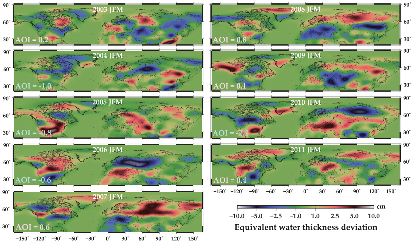
Figure 2. NH maps of wintertime (JFM) equivalent water thickness deviations observed by GRACE. In the lower left corners of the maps are shown AOI corresponding to the green curve in Fig. 1.
