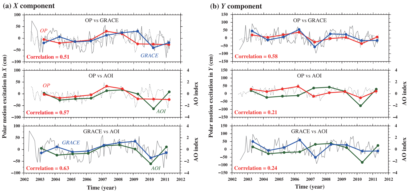
Figure 8. Time-series of the polar motion excitation in (a) X (0E) and (b) Y direction (90E) estimated from the observations of Earth rotation parameters from the Observatoire de Paris (OP) and calculated from mass changes over Eurasia from the GRACE gravimetry. The polar motion observations are based on space geodetic techniques such as the Very-Long-Baseline Interferometry (VLBI). The upper, middle and lower panels compare pairs of OP-GRACE, OP-AOI and GRACE- AOI, respectively. Dashed and solid curves in grey are monthly values of the polar motion excitation from OP (daily values are averaged to monthly values) and GRACE, respectively. Seasonal, linear and quadratic components of these two time-series are removed using least-squares method. Polar motion excitation data are corrected for the geophysical fluid contributions (atmosphere and ocean) available from OP. Blue and red curves are the three months (JFM) averages of the polar motion excitations and GRACE, respectively. Green curves show those of AOI.
