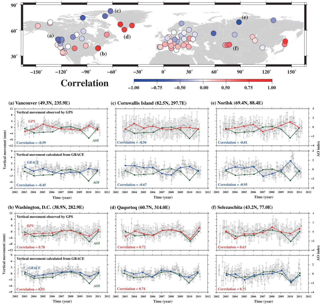
Figure 7. Upper map shows distribution of the correlation coefficients between vertical movement and AO indices at each continuous GPS station. Red dots mean positive correlation and blue dots mean negative correlation. Lower graphs show time-series of vertical movements at (a) Vancouver (49.3N, 235.9E), Canada, (b) Washington, D.C. (38.9N, 282.9E), United States, (c) Cornwallis Island (82.5N, 297.7E), near Northern Greenland, (d) Qaqortoq (60.7N, 314.0E), Southern Greenland, (e) Norilsk (69.4N, 88.4E), near the West Siberian Plain and (f) Selezaschita (43.2N, 77.0E), near the Tien-Shan Mountain Ranges, observed by GPS (upper) and inferred from the GRACE data (lower). Grey dots are monthly values of vertical movement after removing seasonal, linear, and quadratic components. The atmospheric loading contributions are removed from the GPS data using the ECMWF atmospheric model. Blue and red curves are the three-month (JFM) averages of the vertical movements measured by GPS and inferred from GRACE, respectively. Green curves show AOI. Error bars in GPS are one SD and those in GRACE are one-sigma formal errors inferred a posteriori by bringing the chi-square of the post-fit residuals to unity.
