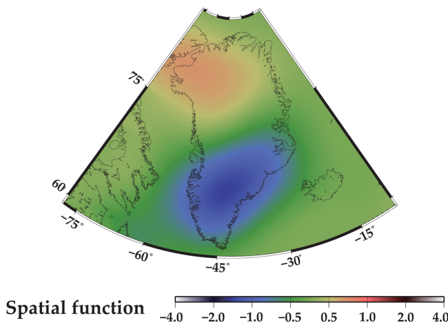
Figure 10. Spatial (left) and temporal (right) functions of the first leading mode derived by the EOF analysis of wintertime mass deviations from GRACE for the three regions, namely (a) Eurasia, (b) North America and (c) Greenland. Black, green, purple and light blue curves are the three-month (JFM) averages of the indices AOI, SOI and PNAI, respectively. Contribution of the first mode was 39 per cent for Eurasia, 47 per cent for America and 44 per cent for Greenland. Time functions in Eurasia and Greenland show high correlations with AOI whereas that in North America resembles more to SOI.
