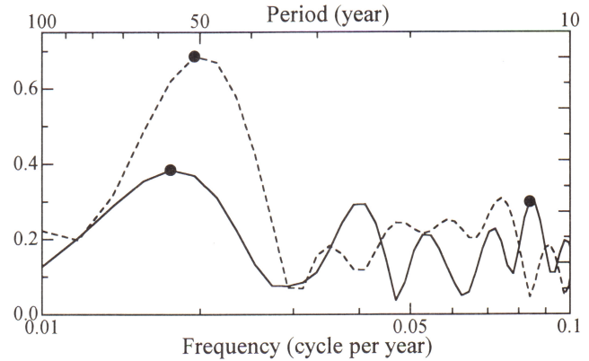
Figure 3. Normalized MTM spectrum of the spring air-temperature in western North America shown in Fig. 1a (solid curve), and spectrum of the winter-spring SLP in the central North Pacific shown in Fig. 1c (dashed curve). A dot indicates a spectrum peak that is significant at the 95% confidence.
